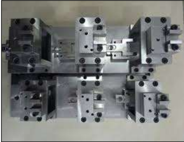
Assembly Jig Fixtures
