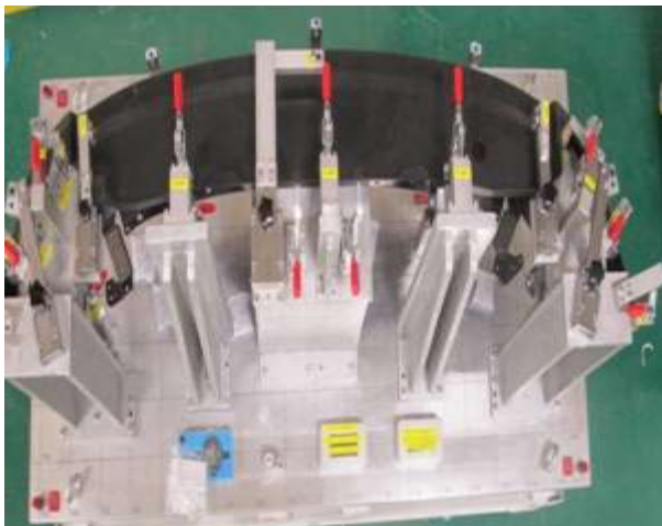
Auto Part Components Jig Fixtures
