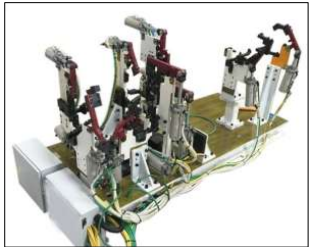
Customized Welding Jig Fixtures
