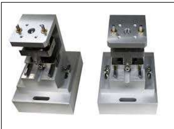
Welding Fixture Sub Assembly
