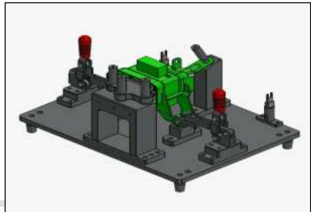
Product Fixtures Assembly
