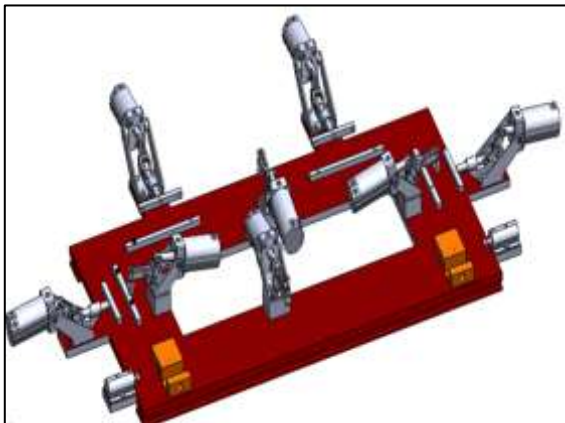
Welding Fixture Sub Assembly
