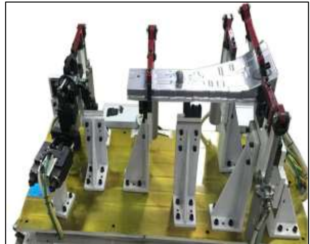
Assembly welding Jig Fixtures
