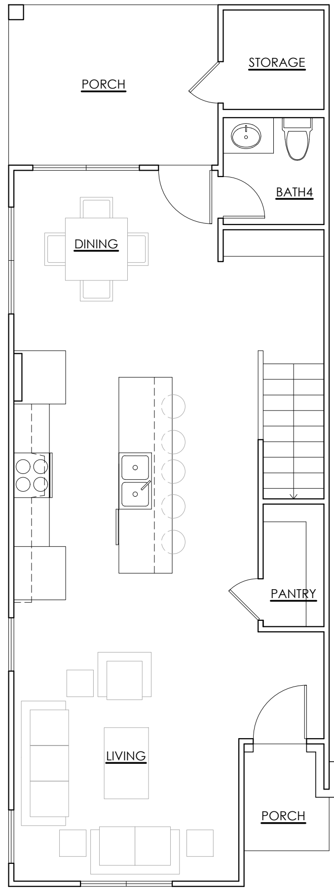
FIRST FLOOR
