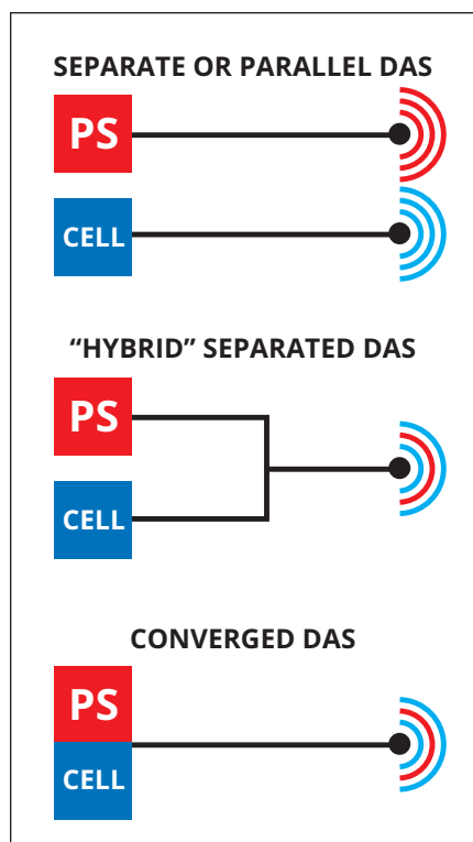
Three approaches for enabling both commercial cellular and public-safety coverage indoors.
